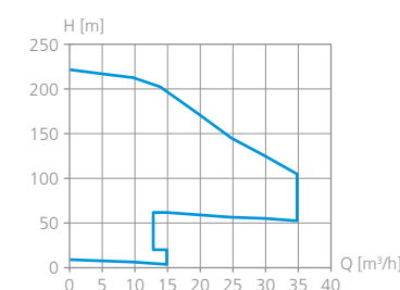
PERFORMANCE CURVE 60 HZ
